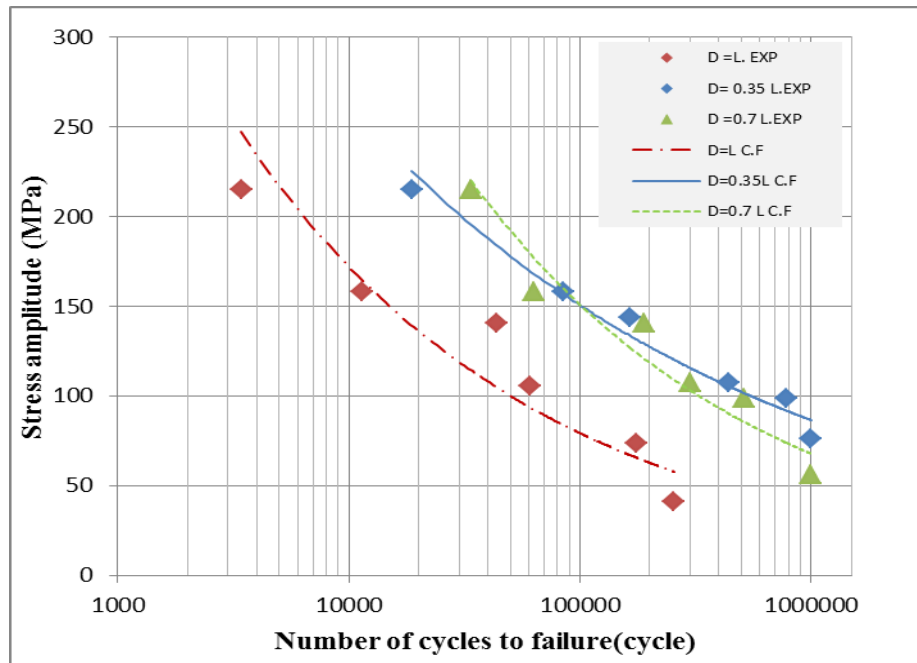
Figure (10) S-N curves for dissimilar 2024T3-6061T6 joints at different welding positions
