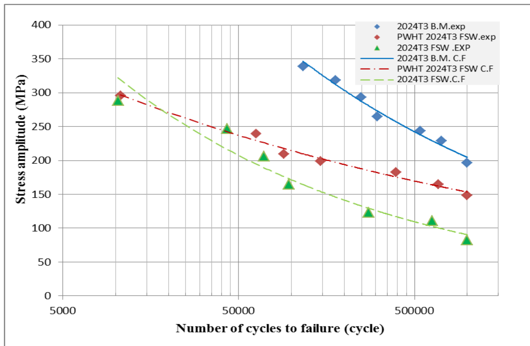
Figure (11) Effect of post welding heat treatment on the fatigue performance
