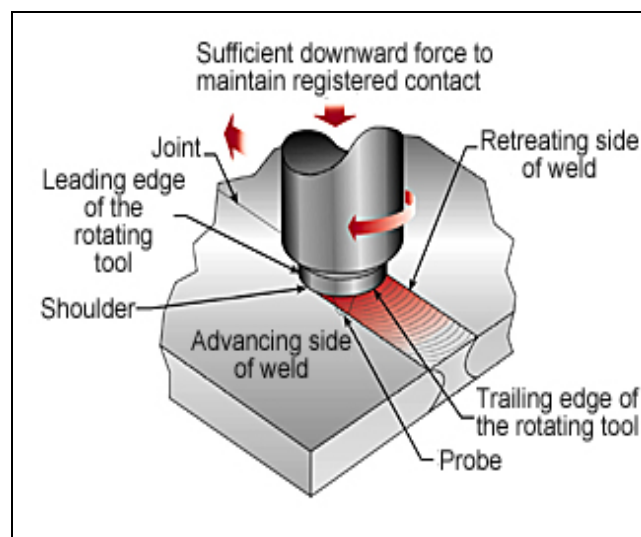
Figure (1) Schematic diagram of the FSW process [2]
