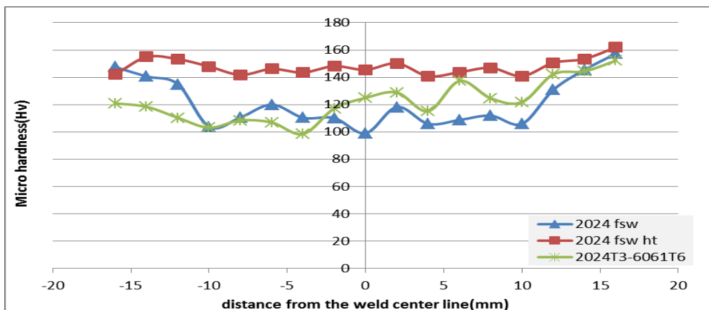
Figure (7) Hardness distribution in similar 2020T3 joints, dissimilar 2024T3-6061T6 joint, and post welding heat treatment 2024T3 joints.
