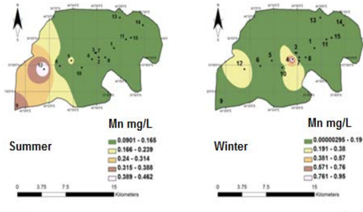
Figure (16): Spatial distribution of Mn concentration in the study area
