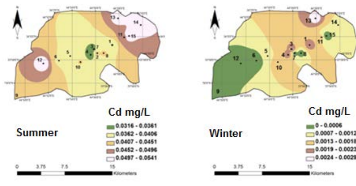
Figure (12): Spatial distribution of Cd concentration in the study area
