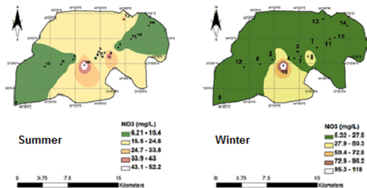
Figure (11): Spatial distribution of NO 3 concentration in the study area
