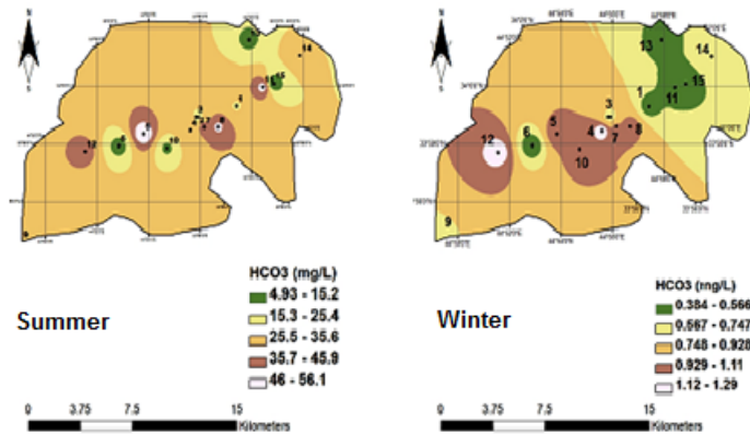
Figure (10): Spatial distribution of HCO 3 concentration in the study area
