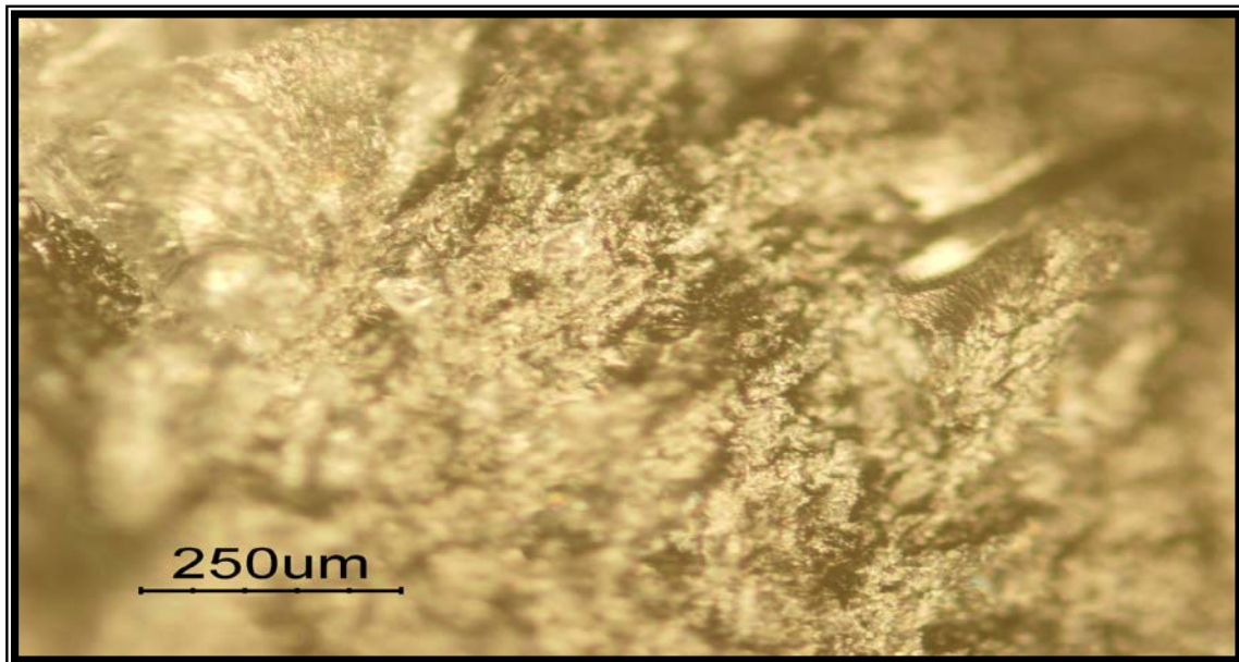
Figure (10) Optical micrograph of fracture surface for (UPE/PS, 90/10%) after impact loading.
