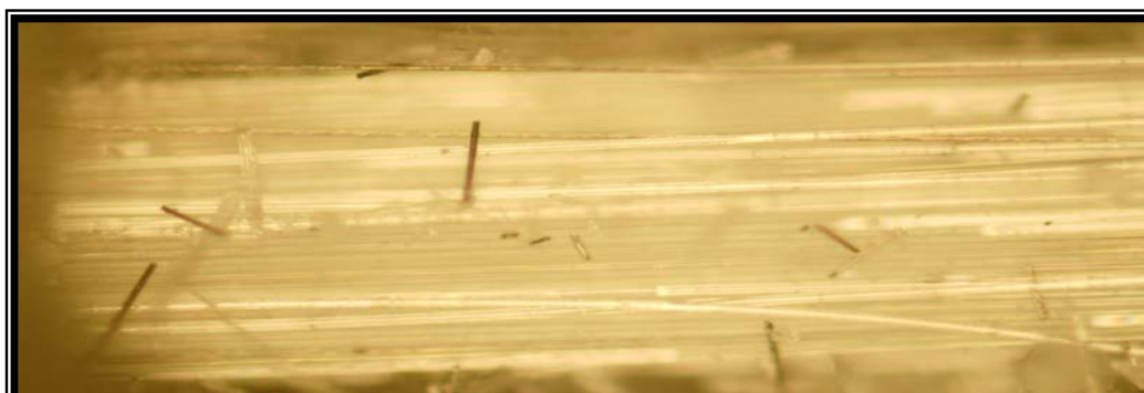
Figure (14) Optical micrograph of fracture surface for (UPE/UP, 80/20%) Polymer blend reinforced with carbon fibers (100X).
