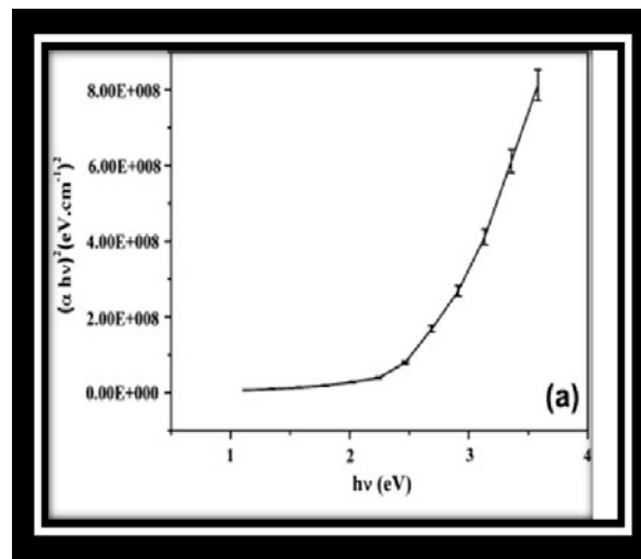
Figure (7) show the relation of (\alpha hv)^2 with the incident photon energy ( hv ).
