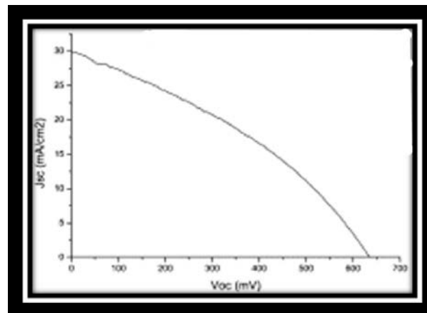
Figure (8) The Photovoltaic Performance of the Cell.
