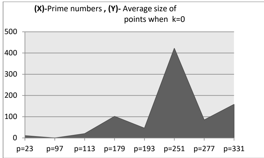
Figure (4) Key space for diffrents prime numbers when k=0.
