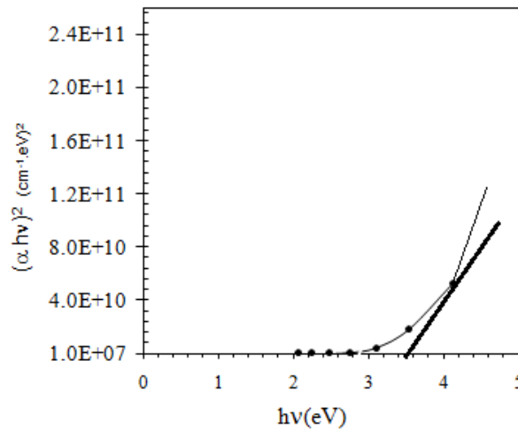
Figure (3) Band gap obtained by extrapolating the linear Portion of the (\alpha hv)^2 versus (hv) curve.
