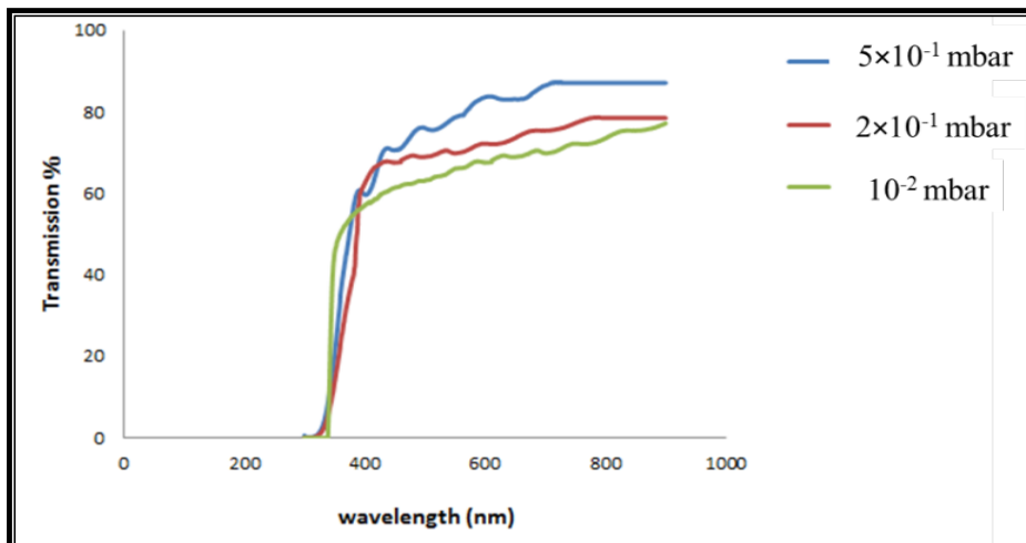
Figure (3):- UV-VIS transmittance spectra of the WO 3 /glass films at different O 2 pressure
