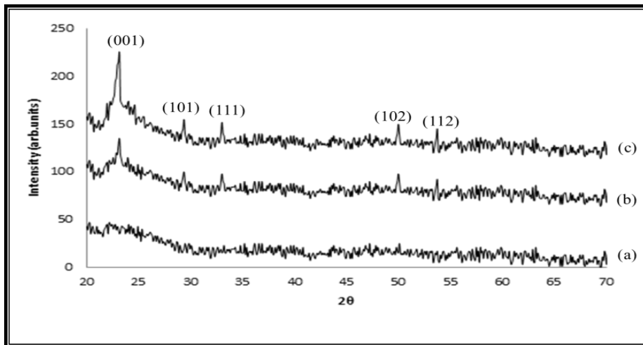
Figure (2):- XRD patterns of WO 3 thin films deposited at various Oxygen pressures a) 10 -2 mbar, b) 2×10 -1 mbar, c) 5×10 -1 mbar
