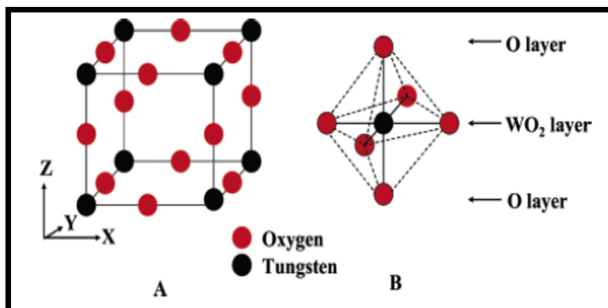
Figure (1):- The crystal structure of WO 3 . (A) The ideal cubic structure of WO 3 . (B) The WO 6 Octahedra in which WO 2 and O planes are alternating [4].
