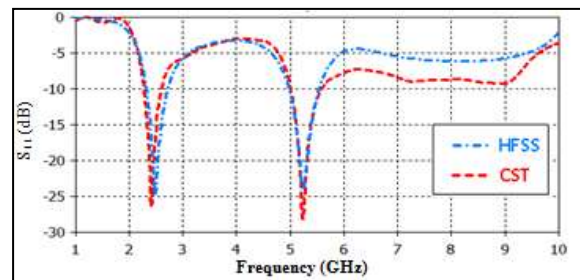
Figure 6: The input reflection coefficient response of the resulting dual-band antenna in CST and HFSS electromagnetic simulators
