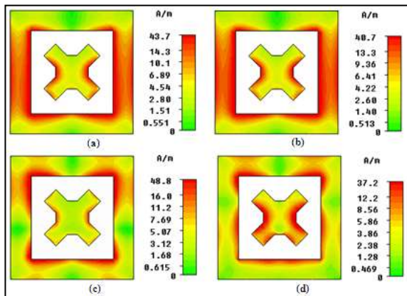
Figure 4: Current distribution analysis on the surface of the triple-band antenna at (a) 2.32 GHz, (b) 2.44 GHz, (c) 4.77 GHz, and (d) 6.72 GHz
