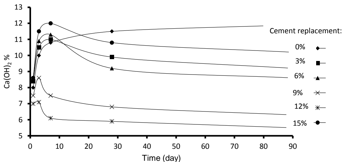
Figure 2: Gradual decrease in \text{Ca}(\text{OH})_2 content due to cement replacement by TAB at different levels [12].
