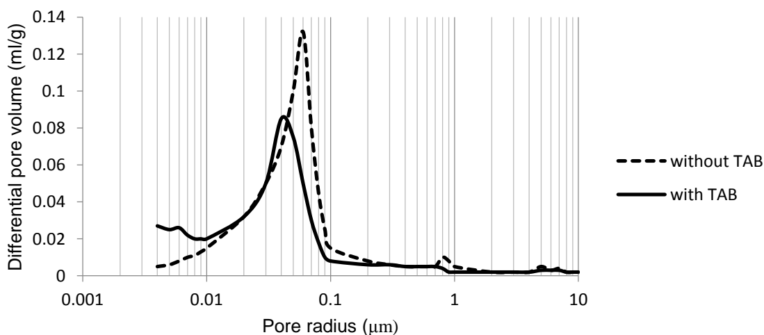
Figure 4: Pore size distributions of 91days old mortars with and without 30% TAB [9].
