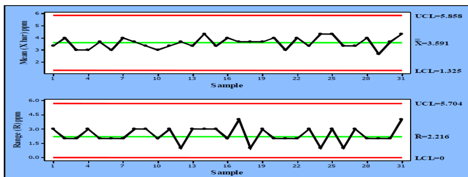
Figure 3: \bar{X} and R charts for gasoline Sulfur content in January/2011
