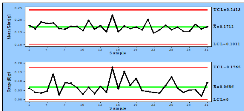
Figure 7: \bar{X} and R charts for gasoline lead additives in January/2011
