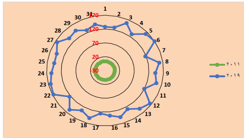
Figure 5: Radar chart for gasoline Sulfur content at years 2011 and 2019
