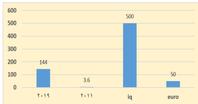
Figure 6: Gasoline Sulfur content compared with IQ and Euro standards
