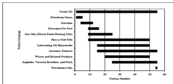
Figure 1: Typical carbon chain lengths [7]
