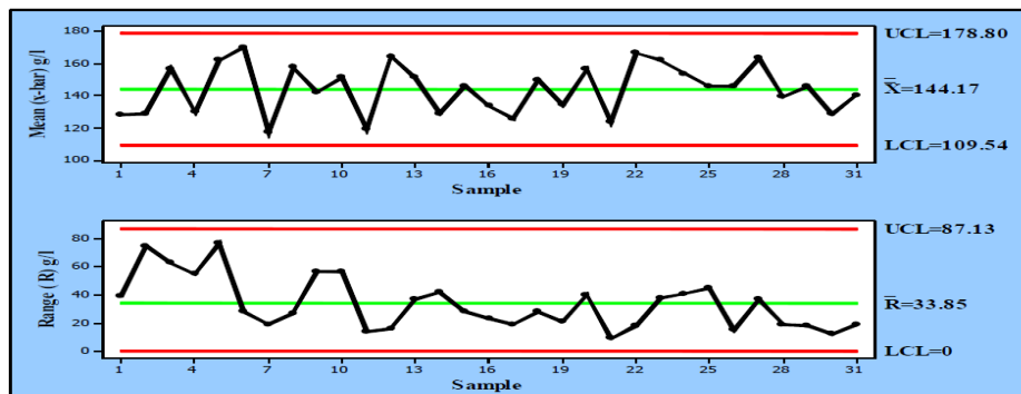
Figure 4: \bar{X} and r charts for gasoline sulfur content in January /2019
