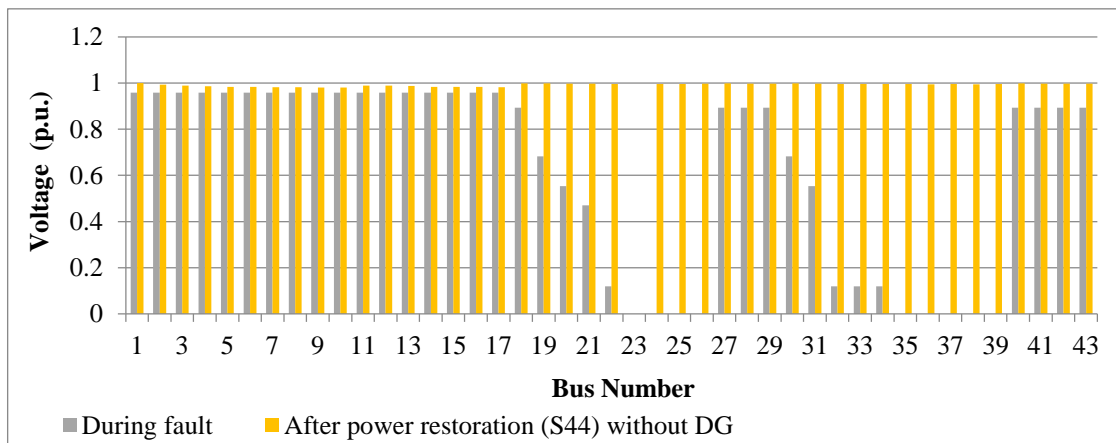
Figure 14: Al-Masbh network voltage profile during fault and after power restoration through (S44)
