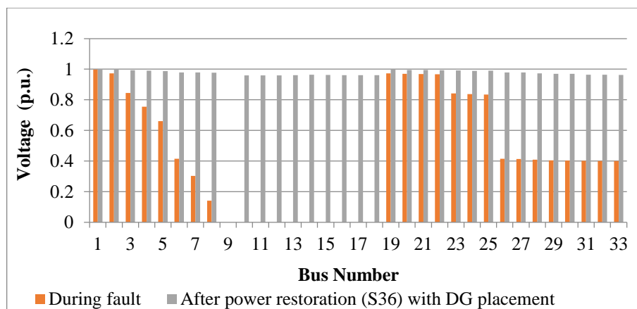
Figure 10: IEEE 33-bus voltage profile during fault and after power restoration through (S36) with DG placement
