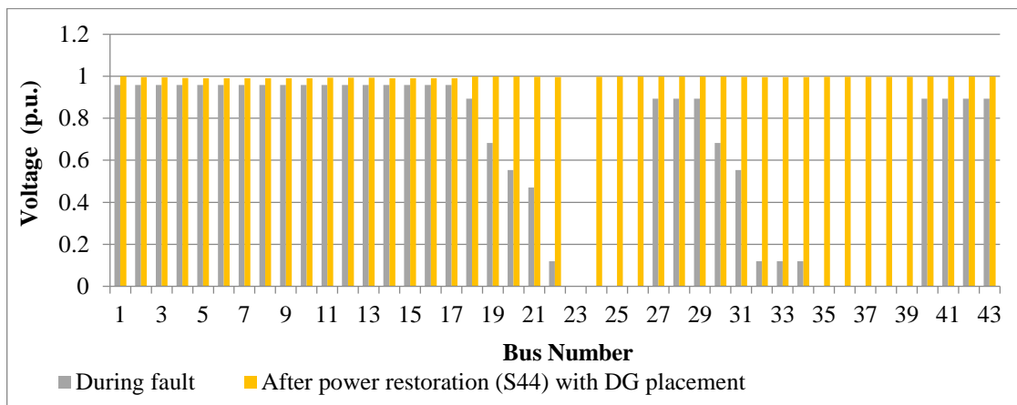
Figure 15: Al-Masbh network voltage profile during fault and after power restoration through (S44) with DG placement
