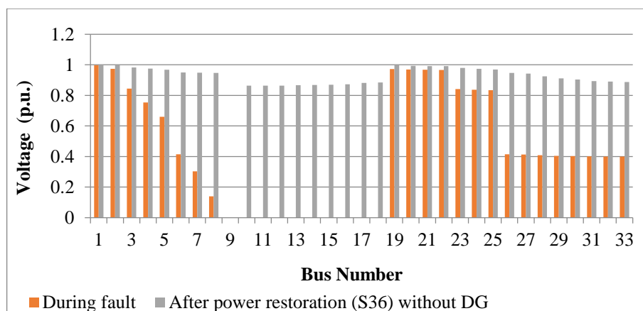
Figure 9: IEEE 33-bus voltage profile during fault and after power restoration through (S36)
