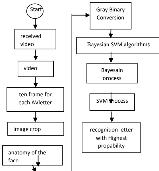
Figure 2: a) Flowchart of the Proposed Bayesian SVM Algorithm for AVletters Recognition, b) GUI The results of this algorithm are shown in Table (I)
