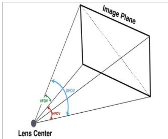
Figure 5: The VFOV, HFOV and DFOV
