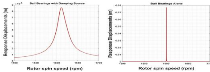
Figure 7: Effect of the external damping source on the response displacement of rotor
