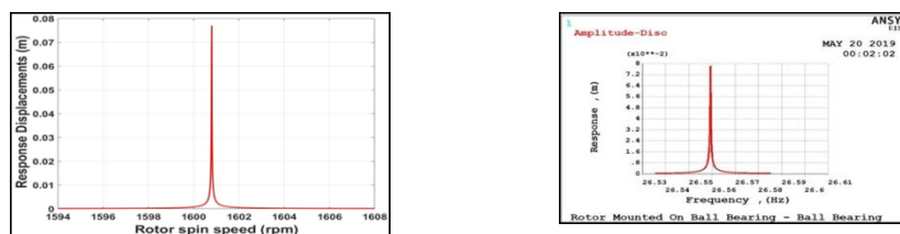
Figure 6: Dynamic response of rotor mounted on ball - ball bearings
