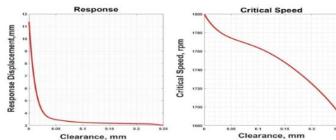
Figure 9: Effect of journal bearing clearance on the critical speed and response
