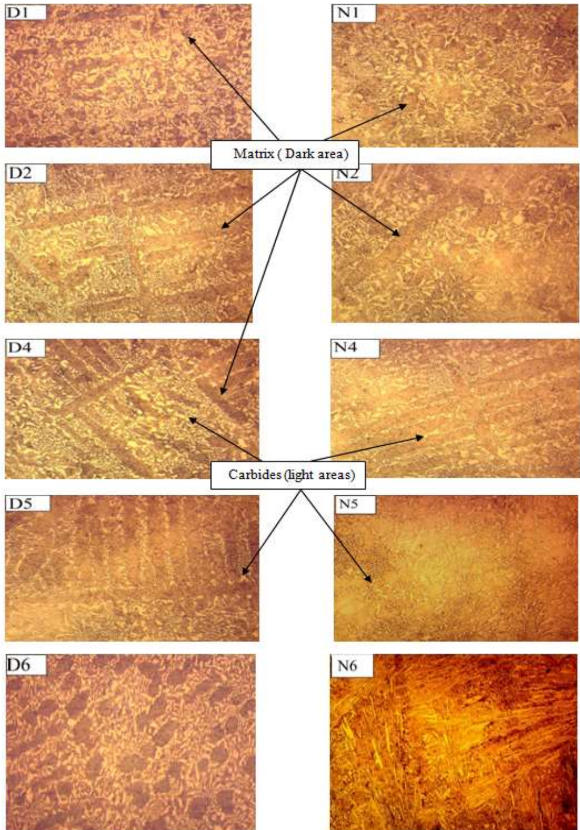
Figure 3: Optical microscope images of the specimens with 20 X magnification
