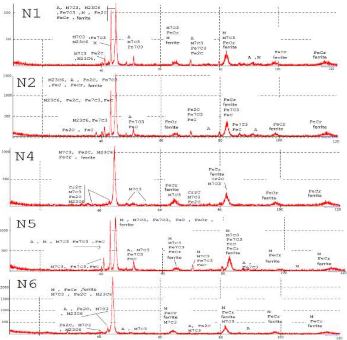
Figure 2: XRD charts of the heat-treated specimens
