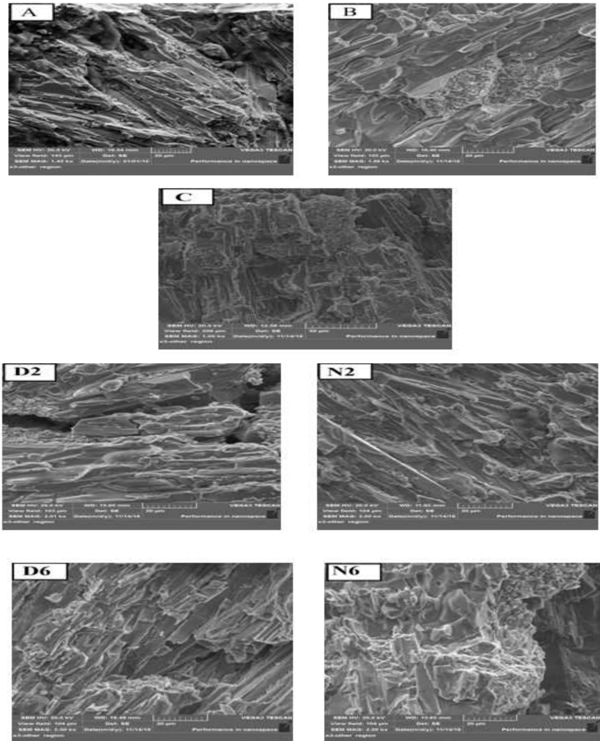
Figure 4: SEM images of different heat-treated samples
