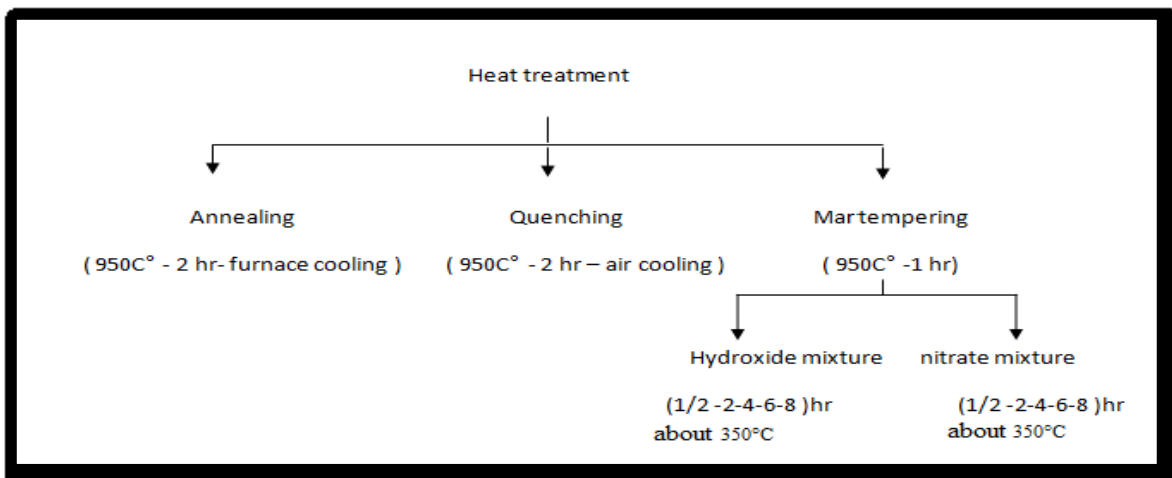
Figure 1-A : heat treatment processes
