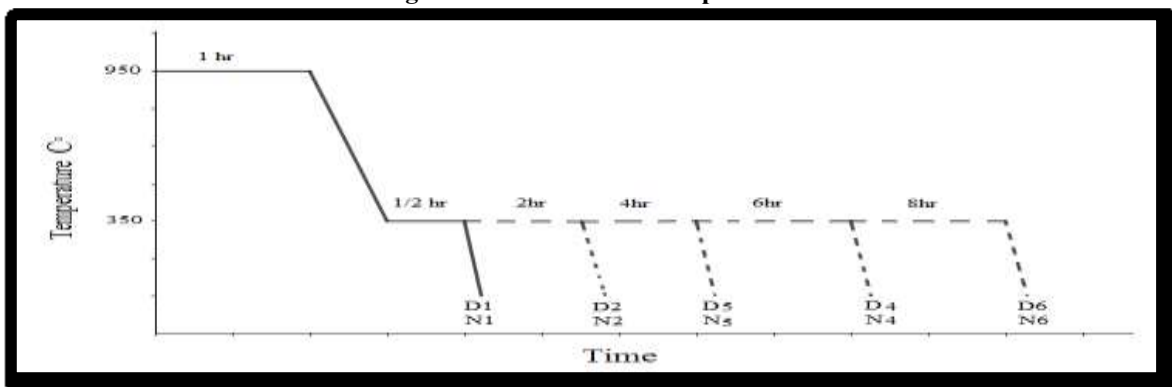
Figure 1-B: Martempering heat treatment procedure
