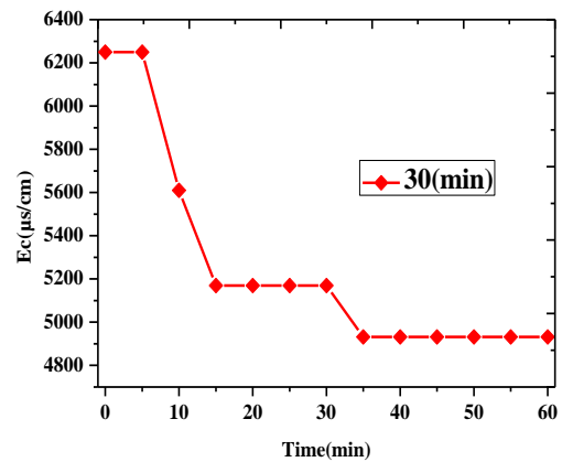
Figure 6 (C): The change in the value of EC with a treatment period of 30 minutes
