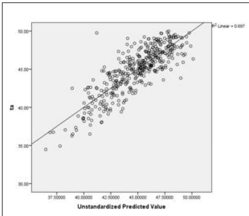
Figure 10: scatterplot of correlation predicted and depended values of air temperature using Modis summer model
