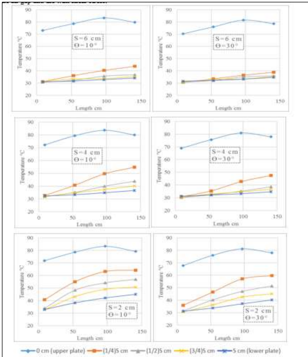
Figure 6: Temperature variation along the length of the channel at 1000 W/m^2 radiation intensity
