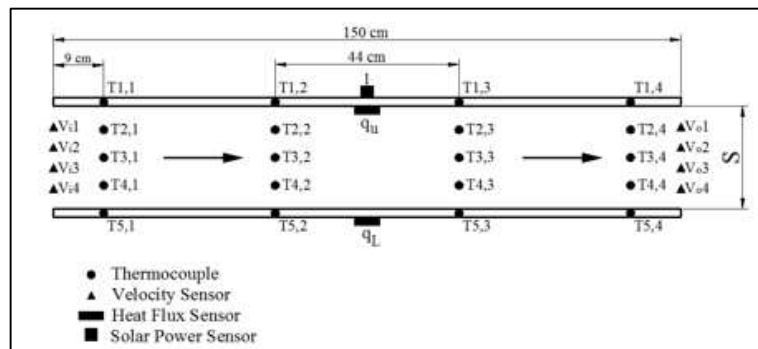
Figure 4: Schematic of sensors distribution in the roof model
