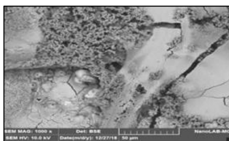
Figure 5: SEM images after corrosion in kerosene medium
