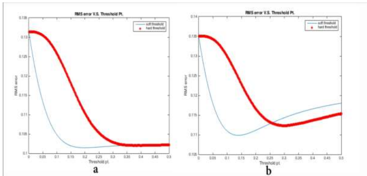
Fig. 4.a.first image example RMS error Vs. soft and hard threshold ( \sigma=0.1 ) b. second image example RMS error Vs. soft and hard threshold ( \sigma=0.1 )
