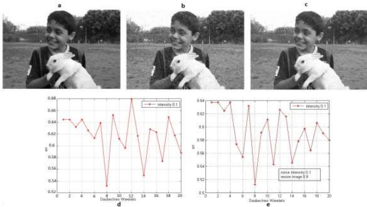
Fig. 2. First image-example of the wavelet( Daubechies function )based denoising: a) original image, b) image with noise ( \sigma= 0.1 ), c) image after denoising procedure with the wavelet db8, d) and e) dependencies of the reconstruction error ( MSE ) versus the number of wavelet for scaling factors 1.0 and 0.9, respectively.
