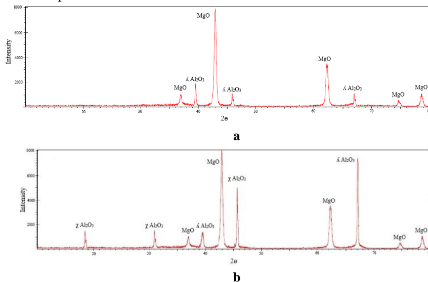
Figure 2: X-ray diffraction patterns for composite nanoparticles (a) The composite nanoparticles (Al 2 O 3 -MgO) with heat treatment at 850 °C. (b) The composite nanoparticles (Al 2 O 3 - MgO) with heat treatment at 550 °C.
