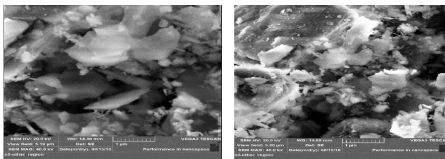
Figure 5: SEM images for the composite nanoparticles. (a) The composite nanoparticles ( \text{Al}_2\text{O}_3 - MgO) with heat treatment at 850 °C. (b) The composite nanoparticles ( \text{Al}_2\text{O}_3 - MgO) with heat treatment at 550 °C.
