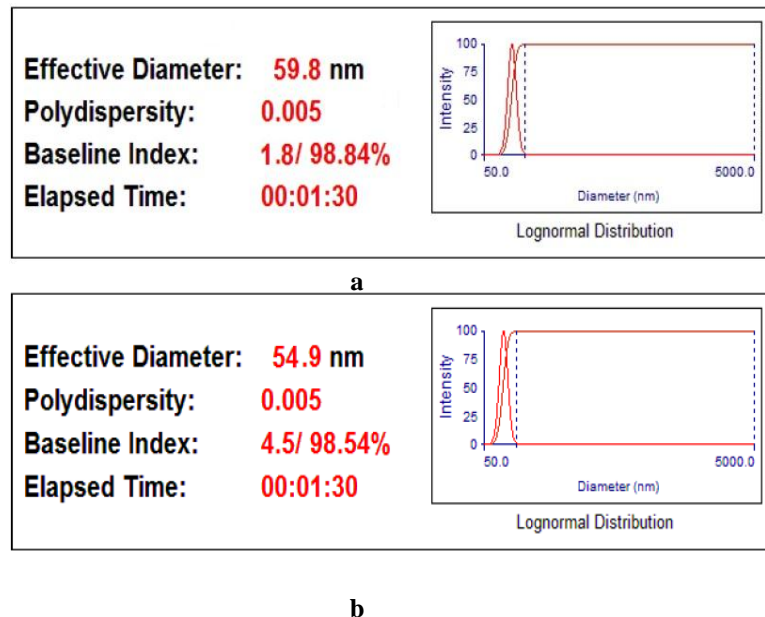
Figure 3: The particle size analysis of the composite nanoparticles. (a) The composite nanoparticles ( \text{Al}_2\text{O}_3 - MgO) with heat treatment at 850 °C. (b) The composite nanoparticles ( \text{Al}_2\text{O}_3 - MgO) with heat treatment at 550 °C.
