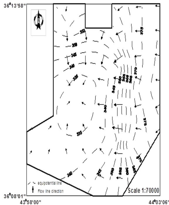
Figure2: levels and movement of groundwater in the study area after [3].
