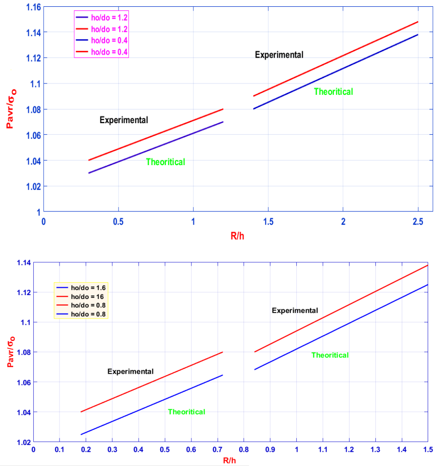
Figure 6: Variation of Pressure Ratio ( P_{avr}/\sigma_o ) with Respect to Radius/Thickness Ratio ( R/h ) for Different Aspect Ratios ( ho/do ) for Solid Cylinder
