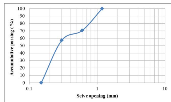
Figure 1: Grading of the natural sand
