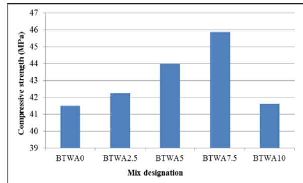
Figure 3: Compressive strength results of black tea waste ash mixes
