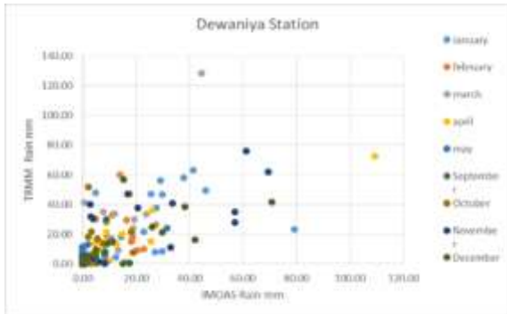
Figure 3: Scatter plot between monthly rainfall data of IMOAS and TRMM in Dewaniya station 1998-2017
