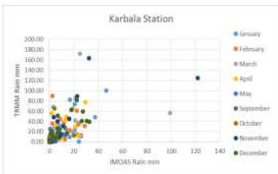
Figure 5: Scatter plot between monthly rainfall data of IMOAS and TRMM in Karbala station 1998-2017
