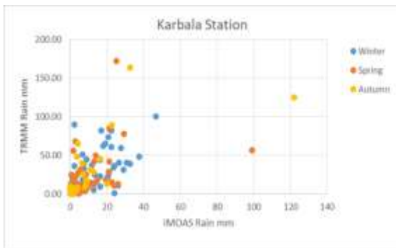
Figure 10: Scatter plot between monthly rainfall data of IMOAS and TRMM in Karbala station 1998-2017
