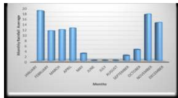
Figure 2: The average of monthly Rainfall (mm) 1998-2017 (IMOAS 2017)
