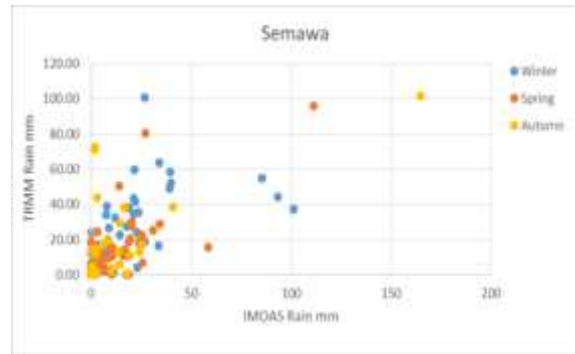
Figure 12: Scatter plot between monthly rainfall data of IMOAS and TRMM in Semawa station 1998-2017
