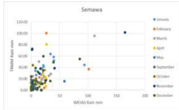
Figure 6: Scatter plot between monthly rainfall data of IMOAS and TRMM in Najaf station 1998-2017
