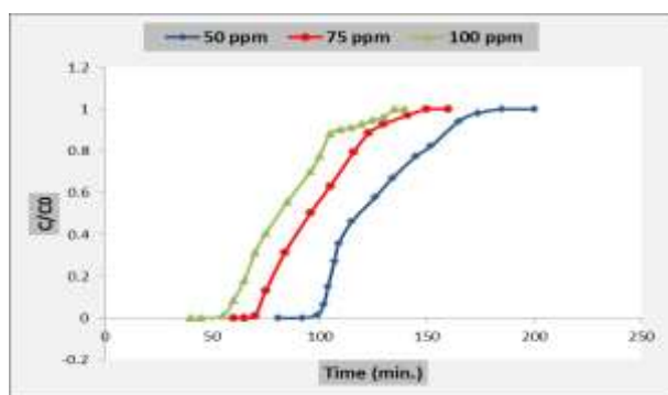
Figure 8: Breakthrough curves for \text{NO}_3^- adsorption on \text{NH}_2\text{-MCM-41} with different \text{NO}_3^- anion concentrations ( Q=1.5 \text{ ml/min} , L=3 \text{ cm} ).
