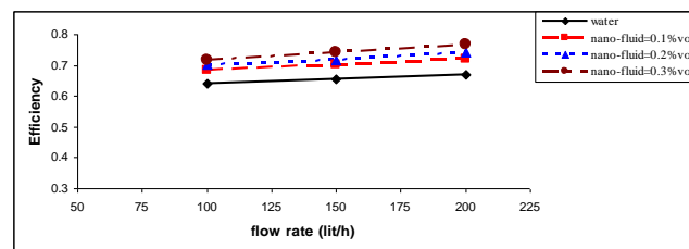
Figure 15: Flow rate and efficiency at different \phi\% of nano-fluid ( \text{SiO}_2 + \text{H}_2\text{O} )
