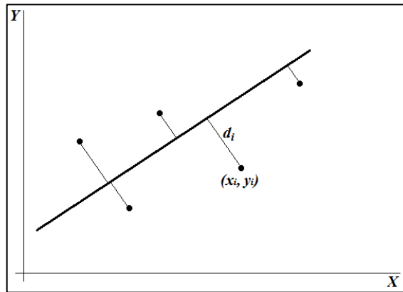
Figure 9: Eigenvector fitting definition for the same set of points of Figure 1.
