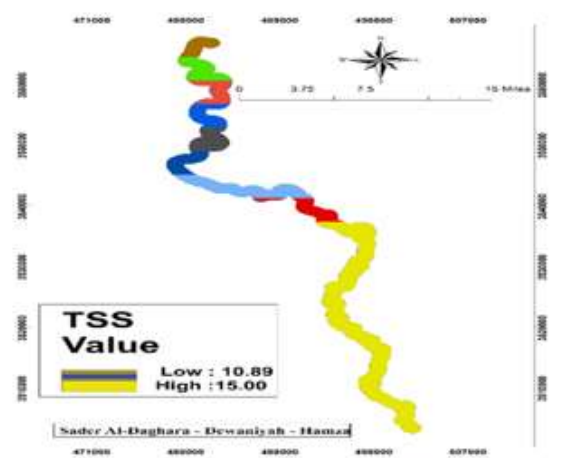
Figure 7: Average TSS values
