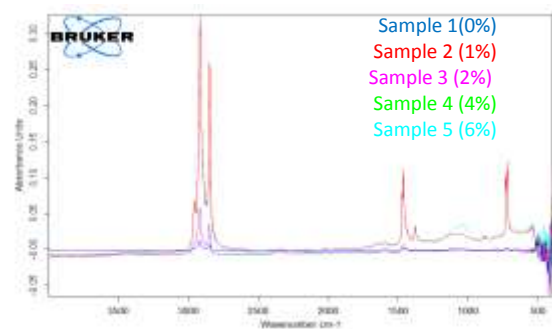
Figure 6: FTIR spectrum of the (nano SiO 2 /wax paraffin) composites
