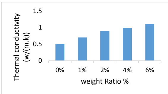
Figure 8: Thermal conductivity of SiO 2 / paraffin wax composite
