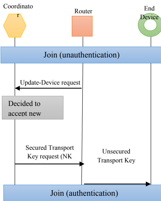
Figure 3. Authentication in standard security method.
