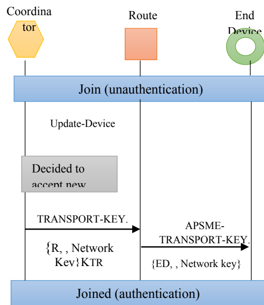
Figure 4. Message arrangement schema (standard security method).
