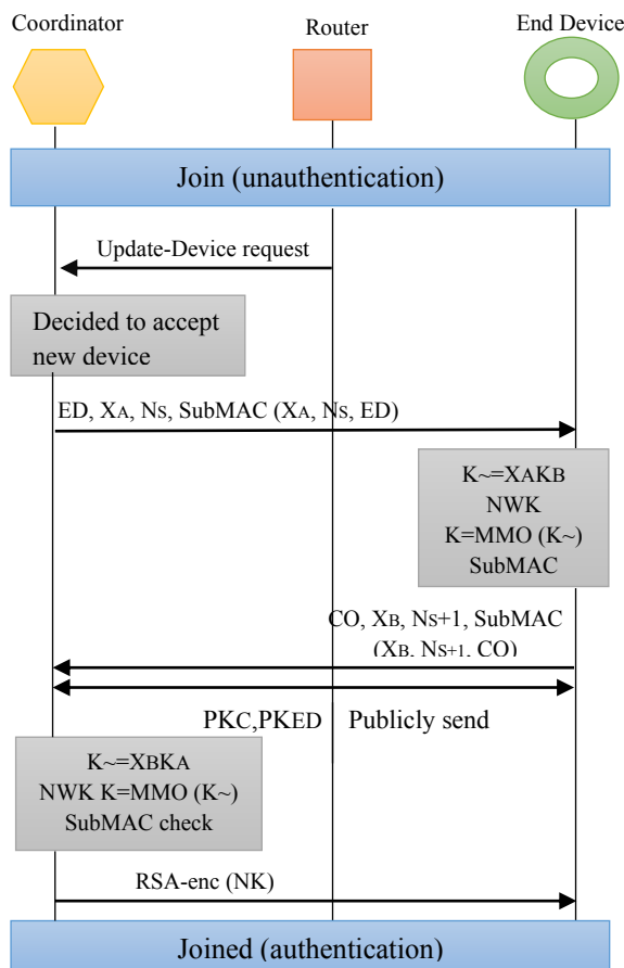
Figure 5. The proposed system to improve security in ZigBee by RSA algorithm.
