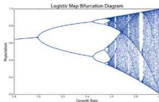
Figure 1. Bifurcation schema of logistic map.
