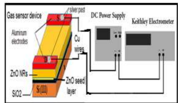
Figure 8: Schematic of a gas sensor device based on ZnO NRs film
