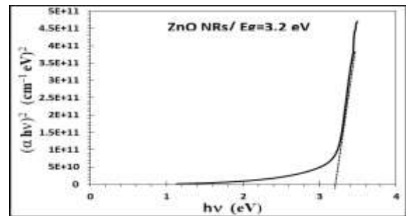
Figure 7: Tauc's plot of optical band gap calculation for the annealed ZnO NRs film
