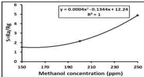
Figure 13: Sensor sensitivity versus methanol concentration.
