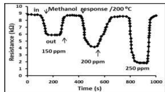
Figure 11: Sensor resistance versus time at various methanol concentrations.
