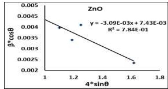
Figure 3: The William-Hall analysis of ZnO NRs grown on silicon
