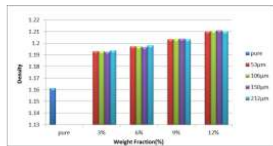
Figure 4: Illustrate the Relationship between the Density and the Weight Fraction of Pistachio shell powder.
