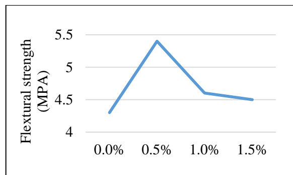
Figure5: Flexural strength of concrete
