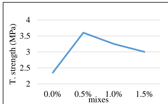
Figure4: Splitting tensile strength of concrete
