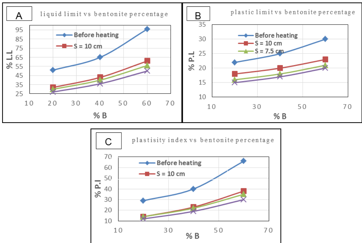
Figure 6: Relationship between liquid limit, plastic limit and plasticity index with bentonite percentages.
