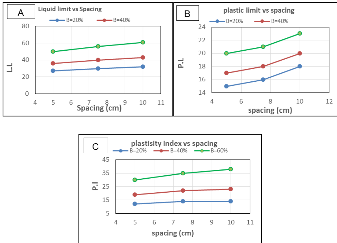
Figure 7: effect of borehole spacing on Atterberg's limit of expansive soil
