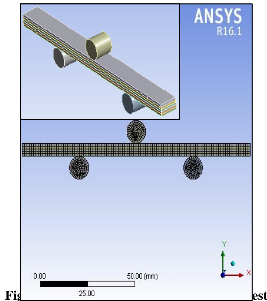
Fig. 1. Finite element analysis model of the nanocomposite beam.
