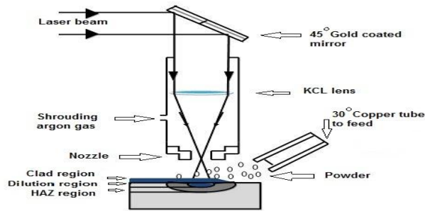
Figure 1: Some laser cladding system components.
