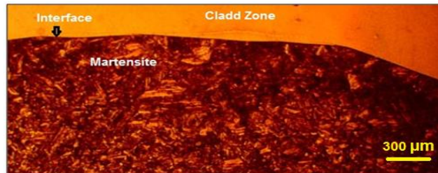
Figure 5: The optical micrograph of the microstructure of martensitic zone.
