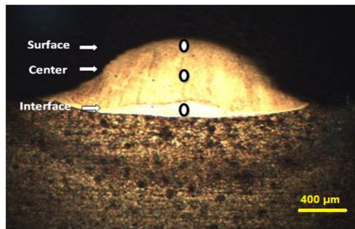
Figure 8: The locations of the applying load in microhardness test.
