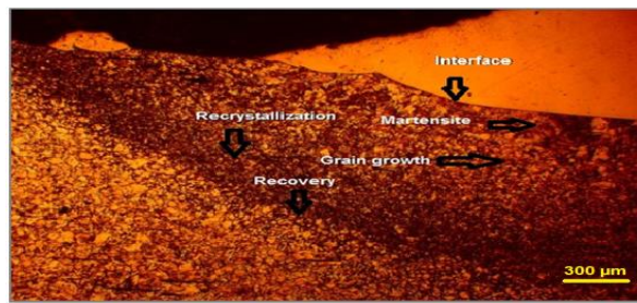
Figure 4: The regions of heat affected zone in addition to the interface.
