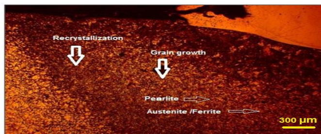
Figure 6: The microstructure comprised of a limited quantity of austenite, ferrite and pearlite.
