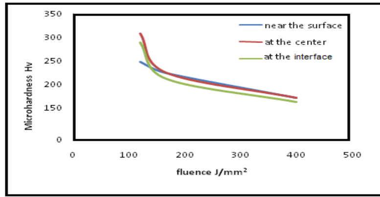
Figure 9: Relationship between microhardness and fluence for all samples groups.
