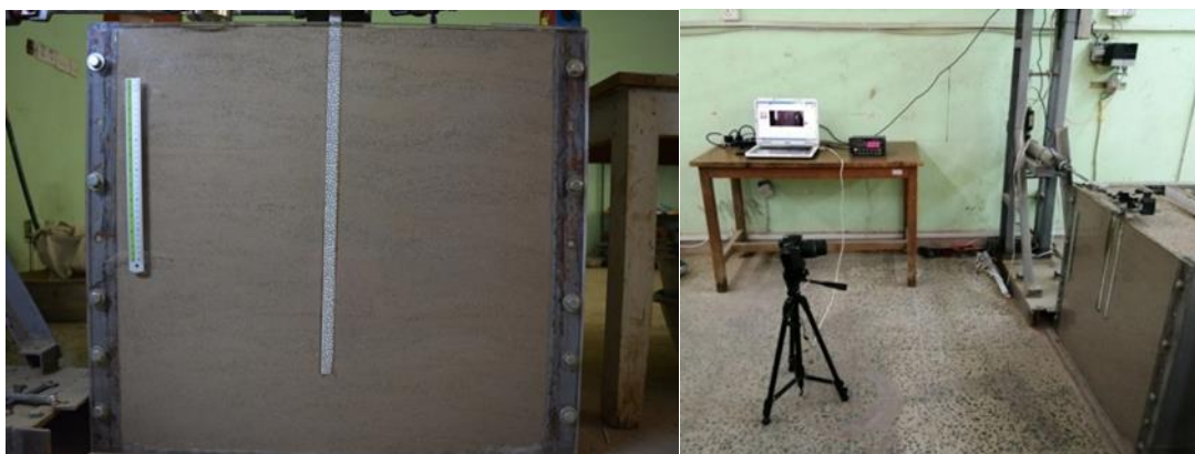
Figure 3: Completed testing model
