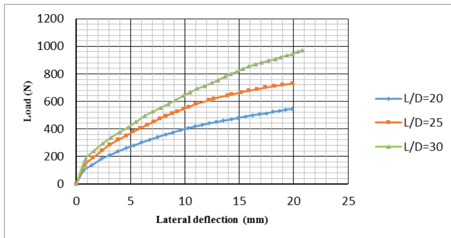
(7): Relationship between lateral load-deflection for group pile of different (L/D) with S/D = 6
