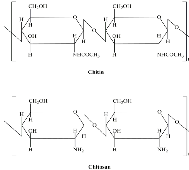
Figure 1: Structure of chitin and chitosan.
