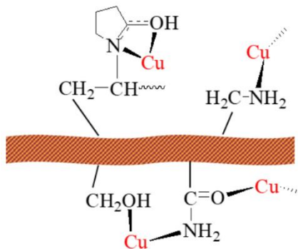
Scheme 1: Possible interactions between Cu(II) ion and crosslinked chitosan
