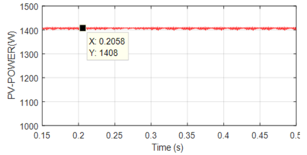
Figure 6: P_{pv} @ 1000W/ m 2 , 60°C R_L (100Ω)
