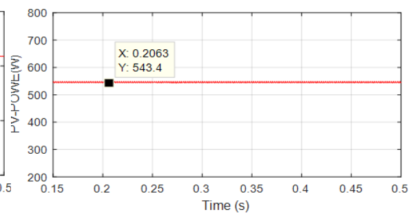
Figure 10: P_{pv} @ 400W/ m 2 , 60°C R_L (200Ω)
