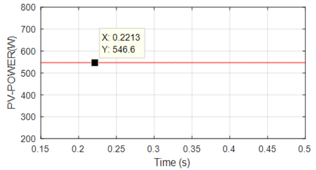
Figure 8: P_{pv} @ 400W/ m 2 , 60°C R_L (100Ω)
