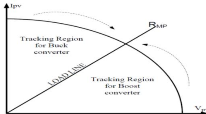
Figure 1: Work reign on I-V curve
