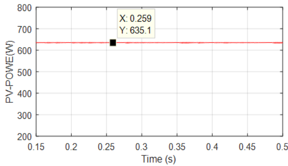
Figure 7: P_{pv} @ 400W/ m 2 , 25°C R_L (100Ω)
