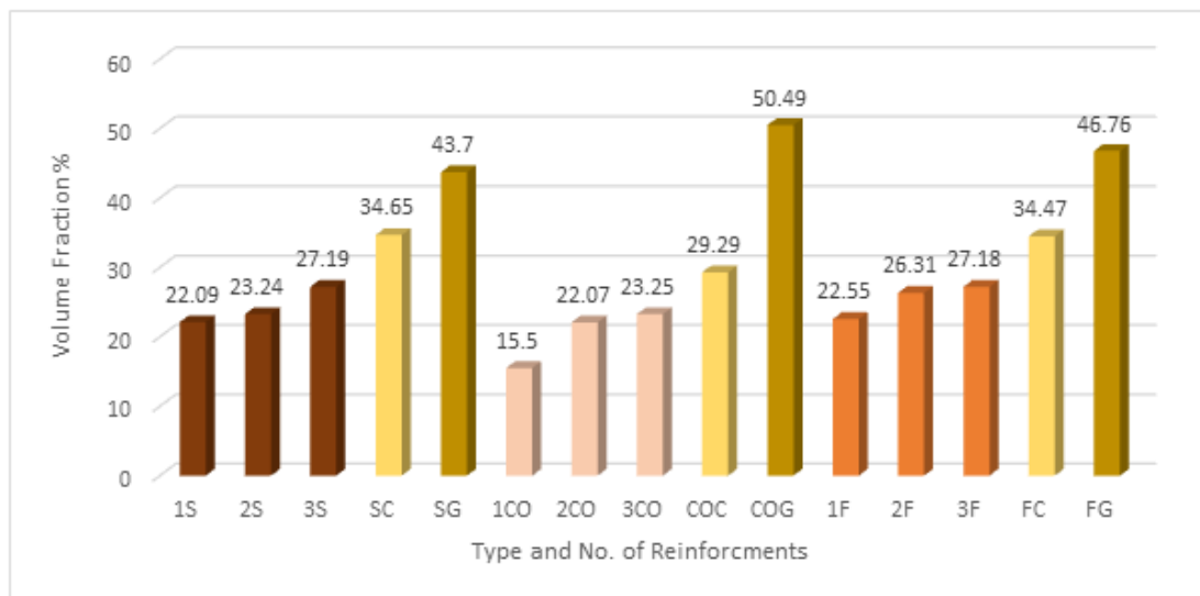
Figure 5: Variation of Volume Fraction of Laminations
