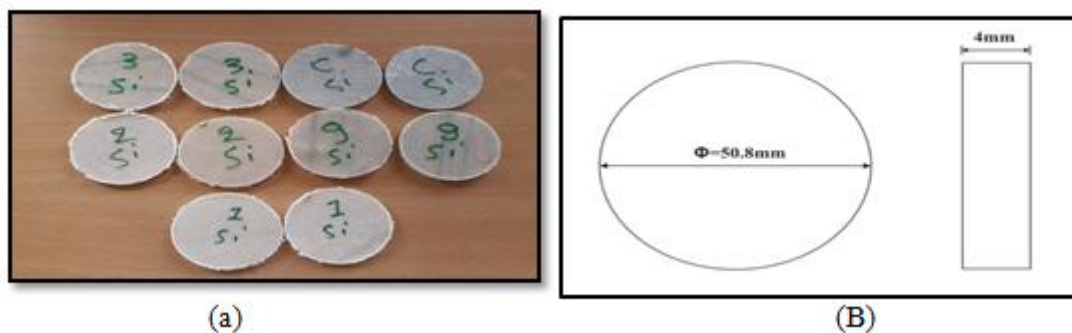
Figure 2: (A) Hardness Test Specimen, (B) Standard Specimen of Hardness Test
