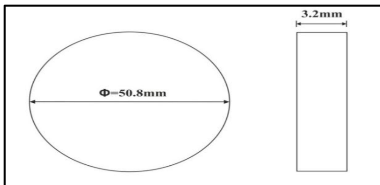
Figure 3: Graphic Sample for Standard Specimen of Water Absorption Test
