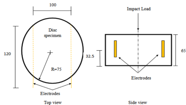
Figure 5: Geometrical details of electrodes (all dimensions are in mm)
