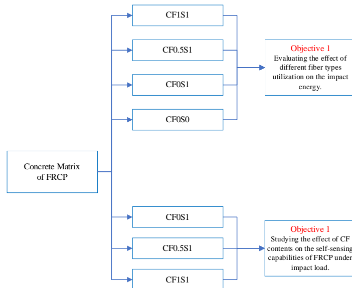
Figure 1: Flow chart of the experimental program
