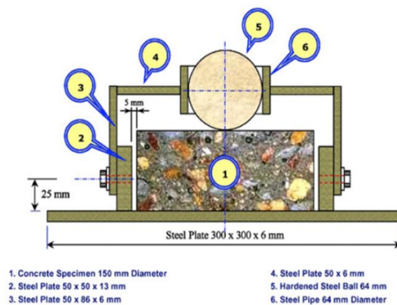
Figure 4: Impact test setup [55]
