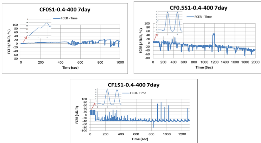
Figure 8: Effect of carbon fibers utilization on the average FCER results under impact load for different mixtures
