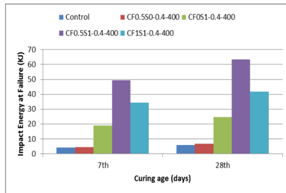
Figure 7: Effect of different fibers utilization on the average impact energy results
