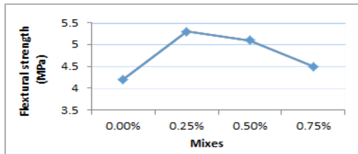
Figure 6: Flexural strength of Silica Fume concrete
