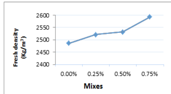
Figure 3: Fresh density of Silica Fume concrete
