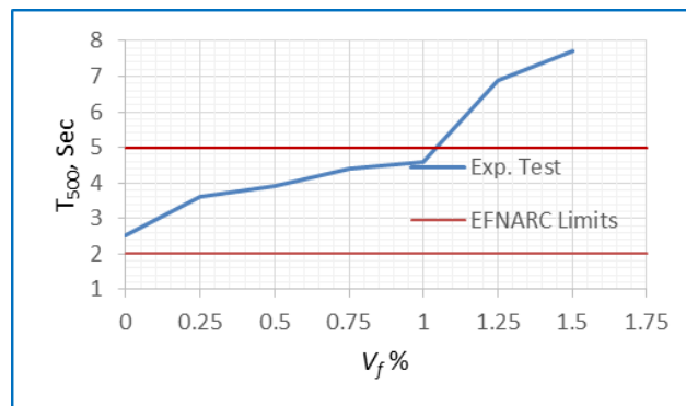
Figure 2: Steel volume fraction versus T 500 test
