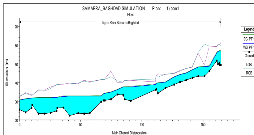
Figure 5: Reach in steady state with Mix discharge (Q=638.17m3/sec).Appendix
