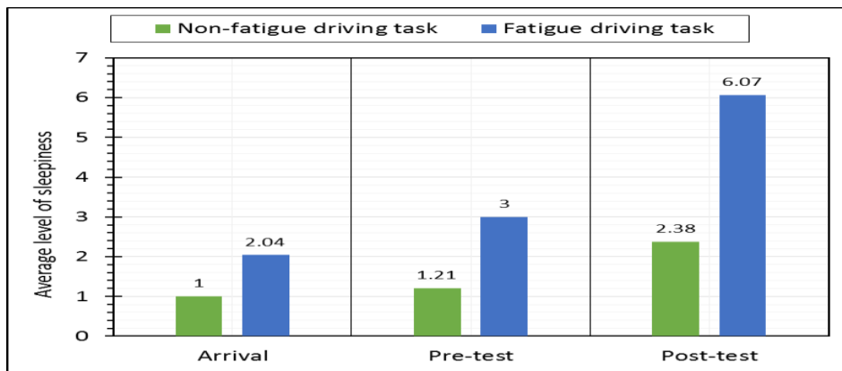
Figure 5: Change in mean Stanford sleepiness scale score for all participants and both tasks
