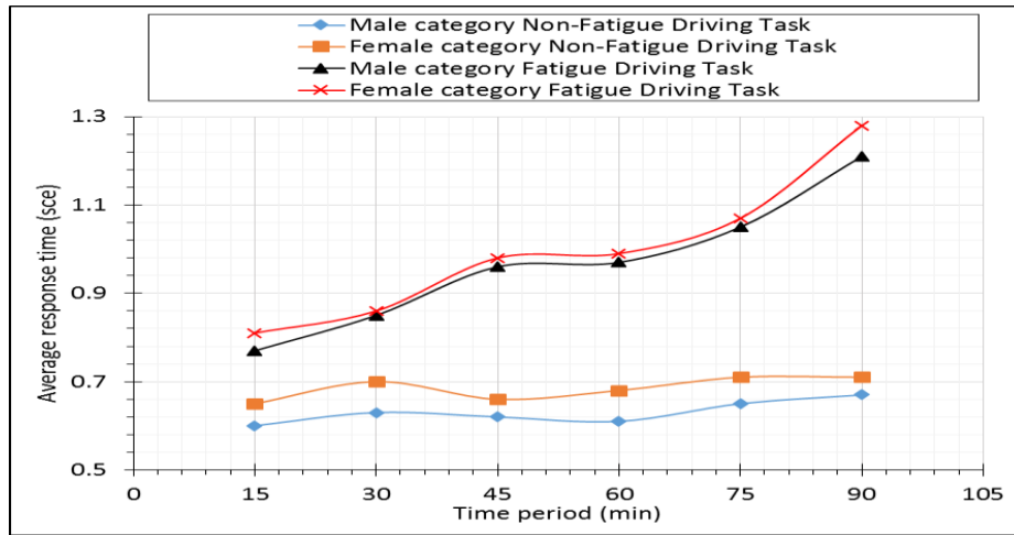
Figure 7: Change in the average response time for gender
