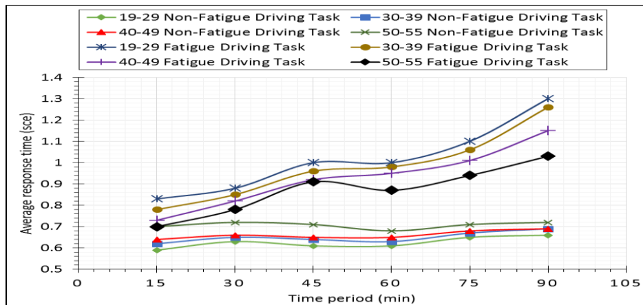
Figure 8: Change in the average response time for Age groups
