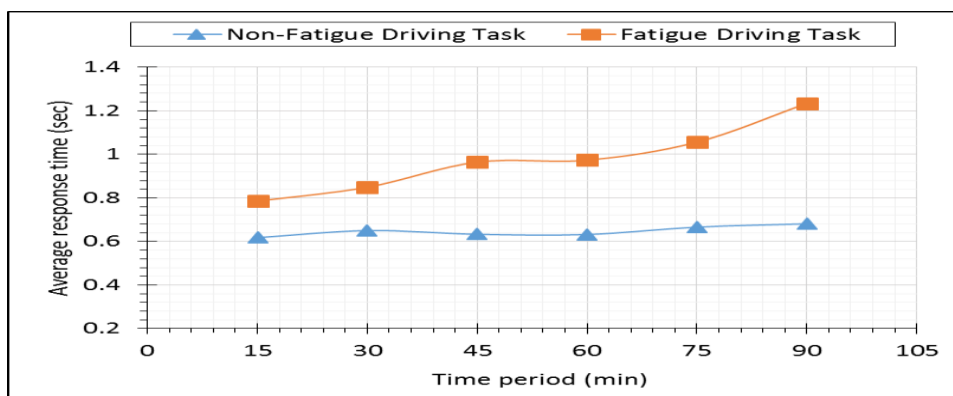
Figure 6: Change in the average response time for all participants
