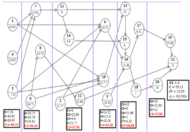
Figure 8: Distributing of tasks among the workstations in the line based on the MSLO method
