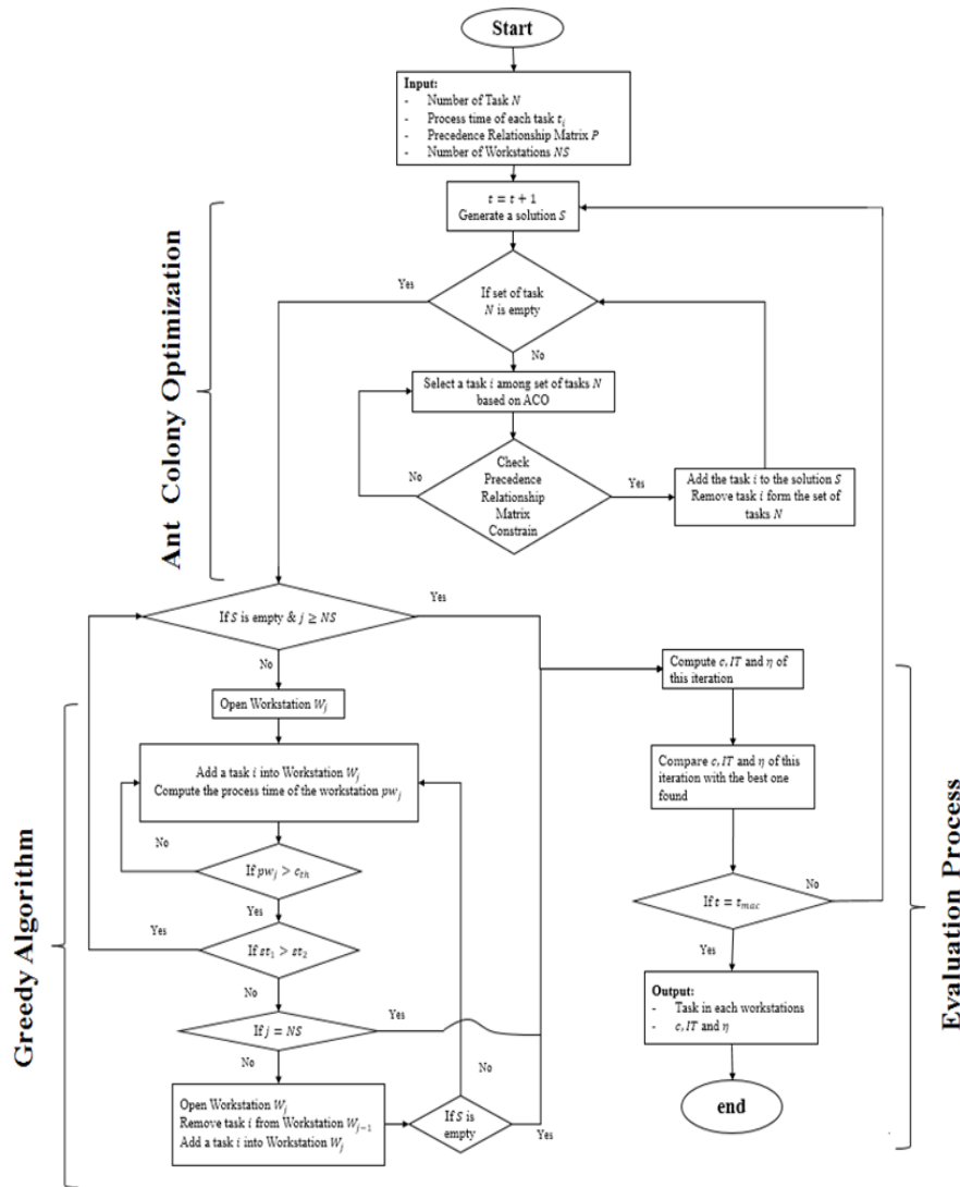
Figure 2: Structure of the Ant-Greedy optimization
