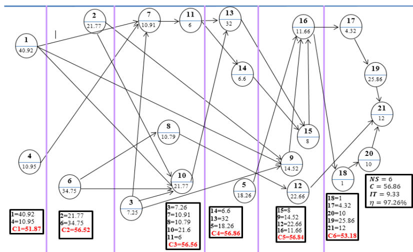
Figure 9: Distributing of tasks among the workstations in the line based on the Ant-Greedy optimization method
