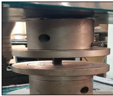
Figure 3: Compression test device
