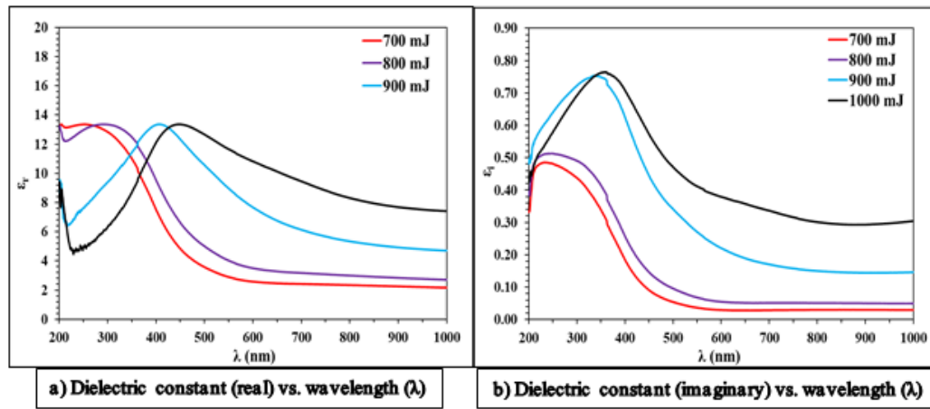
Figure 7: Fe 3 O 4 at different laser energy
