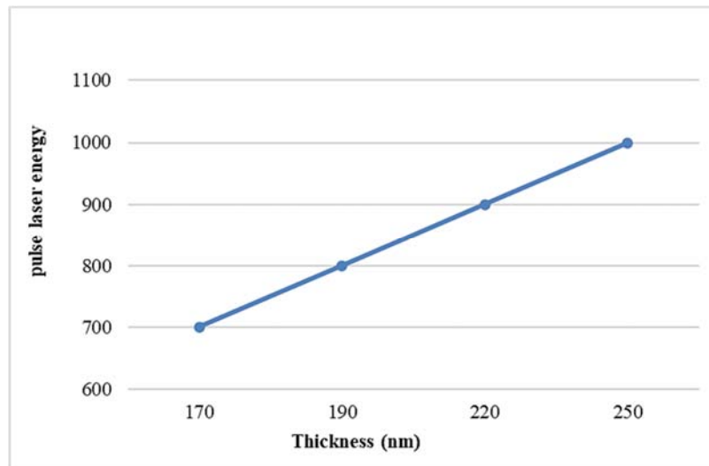
Figure 8: The thickness of Fe 3 O 4 thin films for different pulse laser energies
