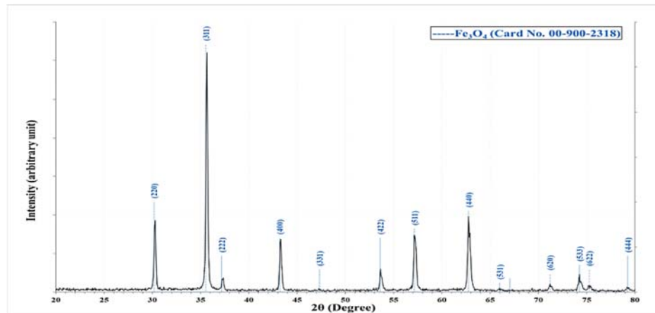
Figure 3: XRD pattern of Fe 3 O 4 powder
